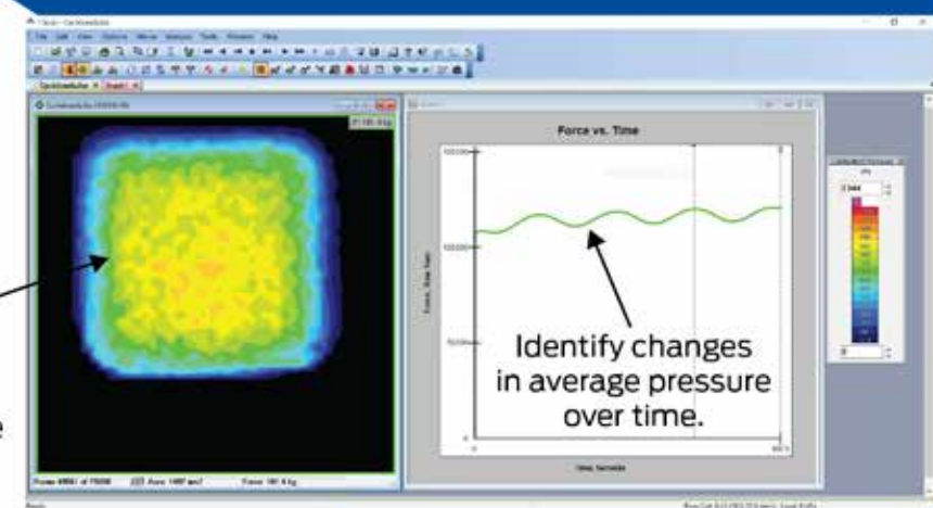
Blue-to-red color scale identifies regions of variable pressure across the battery pouch.
